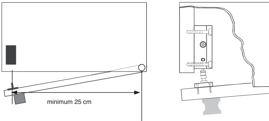
Illustration 7: Mounting to a cabinet
