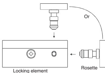
Illustration 1: Locking principle
