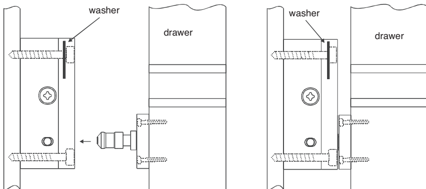
Illustration 6: Mounting to a drawer
