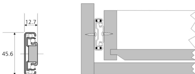
Installation Diagram
