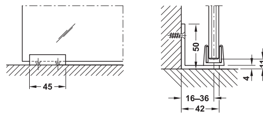
Section floor guide
