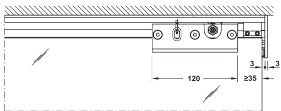
Section trolley hanger 40-50 kg
