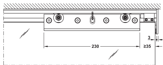
Section trolley hanger 80-120 kg
